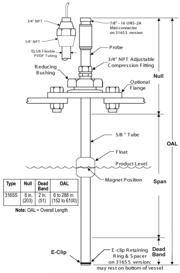
Typical Installation
