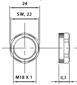
plastic clamping ring (2x included in delivery)
