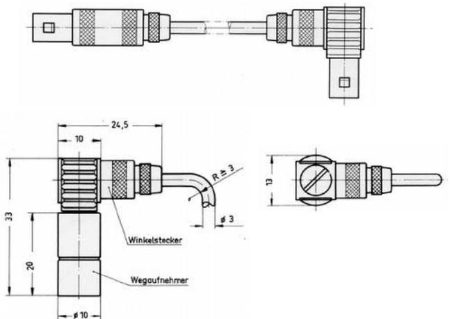
Dimensions with sensor K0100
